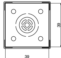
N51-25 BGA 38 x 38
