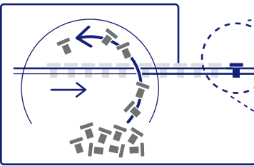
通过磁力可稳定输出螺丝到轨道上 Magnetically conveys screws along rails for a stable feeding
