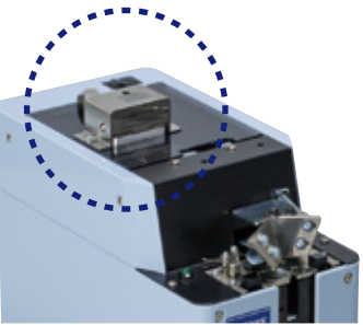
通过磁力可稳定输出螺丝到轨道上 Magnetically conveys screws along rails for a stable feeding
